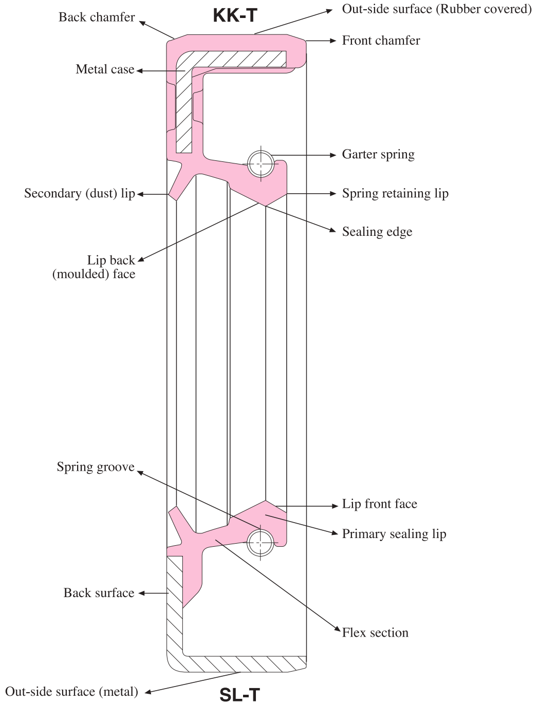
Figure 1: Terminology of radial shaft seals (with spring-loaded lip)
