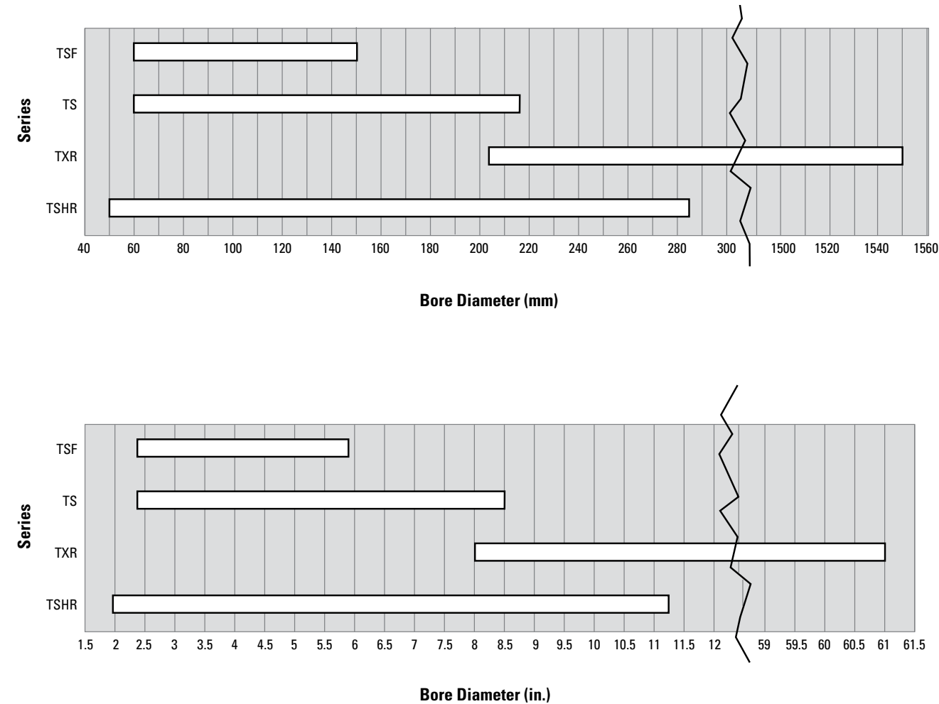
Fig. 109. Bore diameters.
