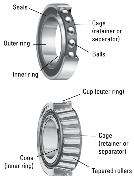
Fig. 2. Bearing components.
