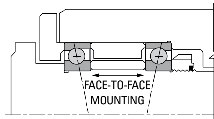
Fig. 87. DF Mounting, fixed (not suggested).
