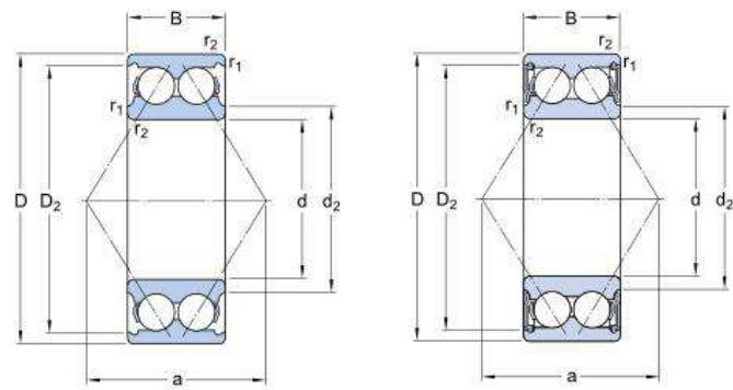
Double Row Angular Track Well – open and closed type
