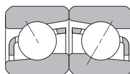
Face-to-face arrangement (DF)
